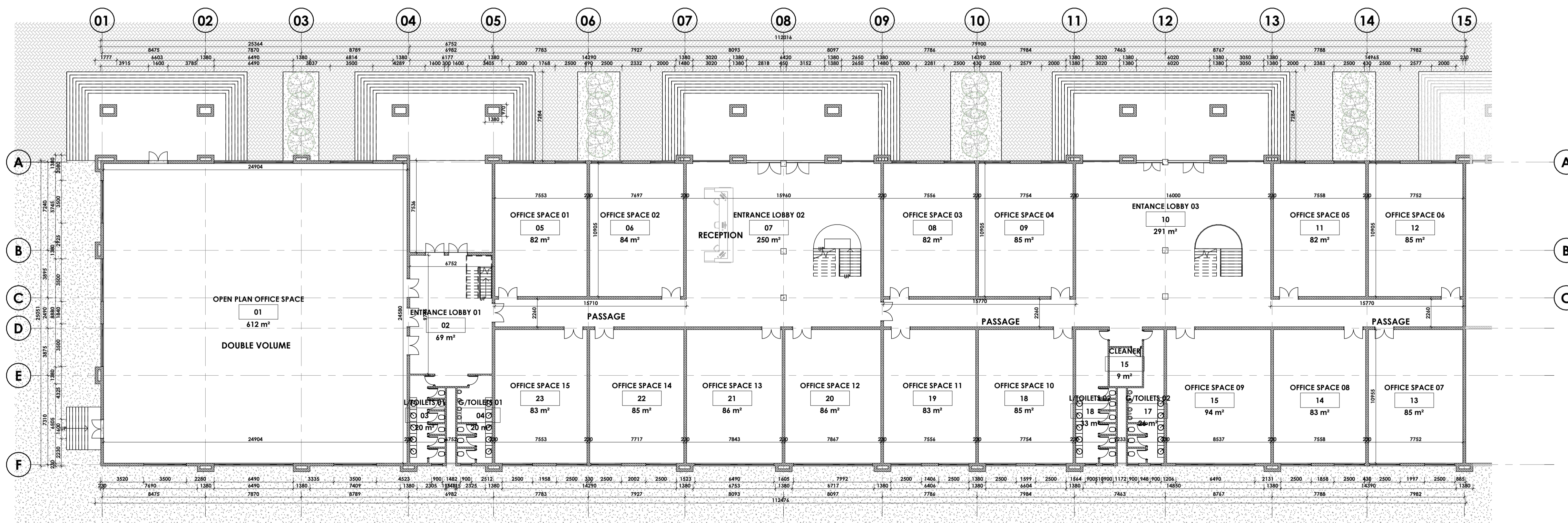
2 01.Ground Floor Plan 1 : 200
