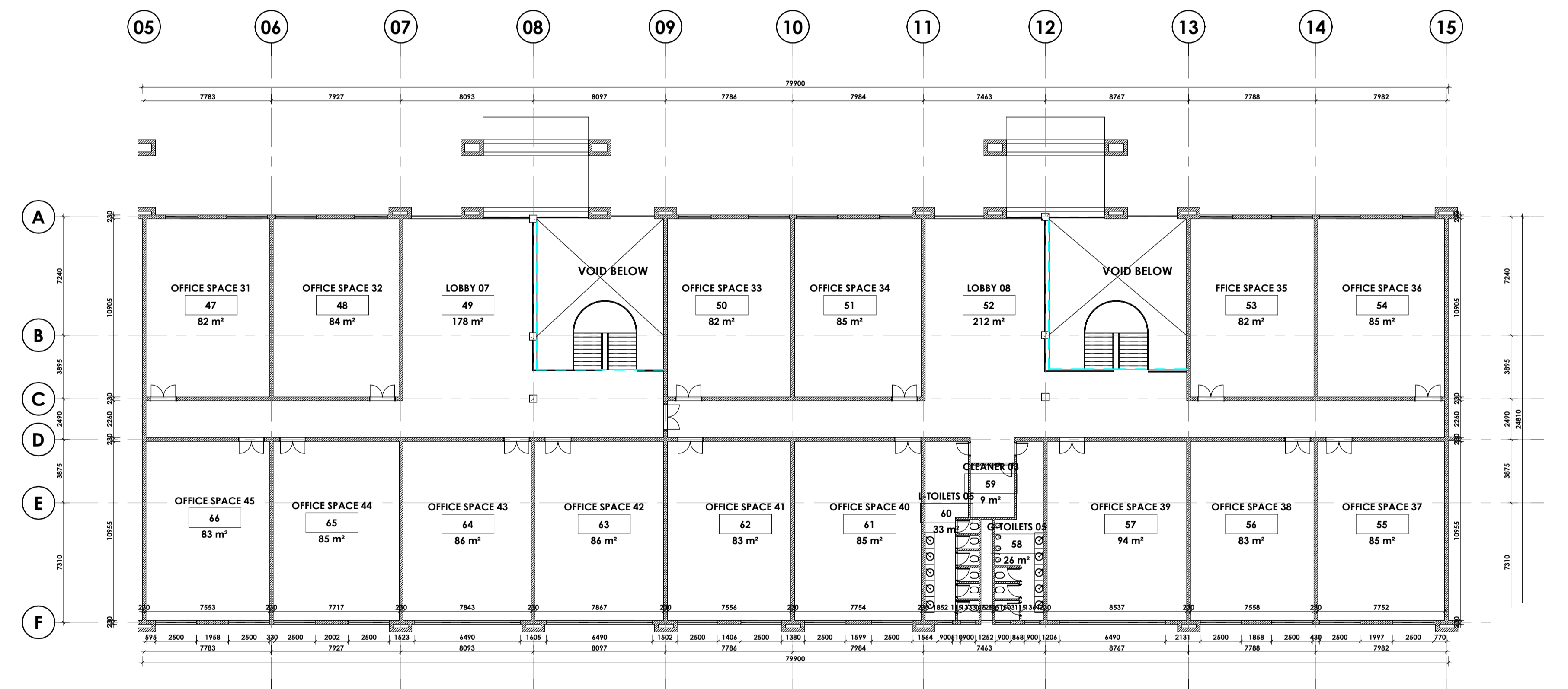
3 05.Second Floor Level 1 : 200
